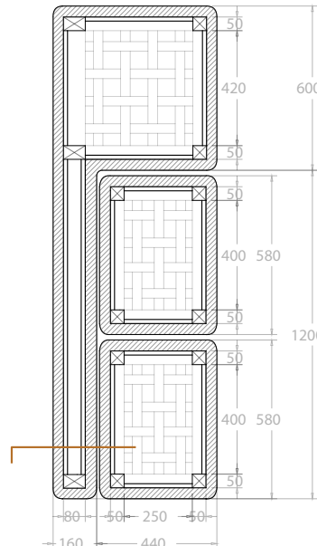
PLAN SECTION
