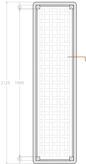
PLAN SECTION
